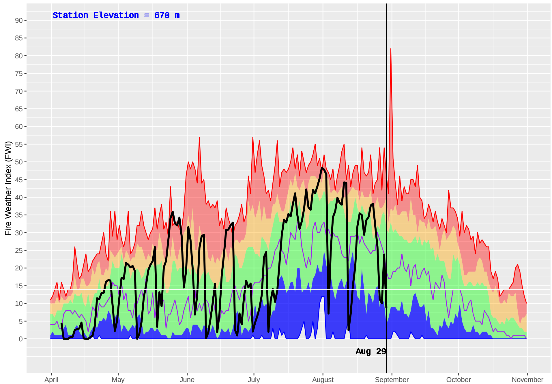
FINTRY (298) : Historical (1989–2016) and Current (2018) Daily Fire Weather Index (FWI)
