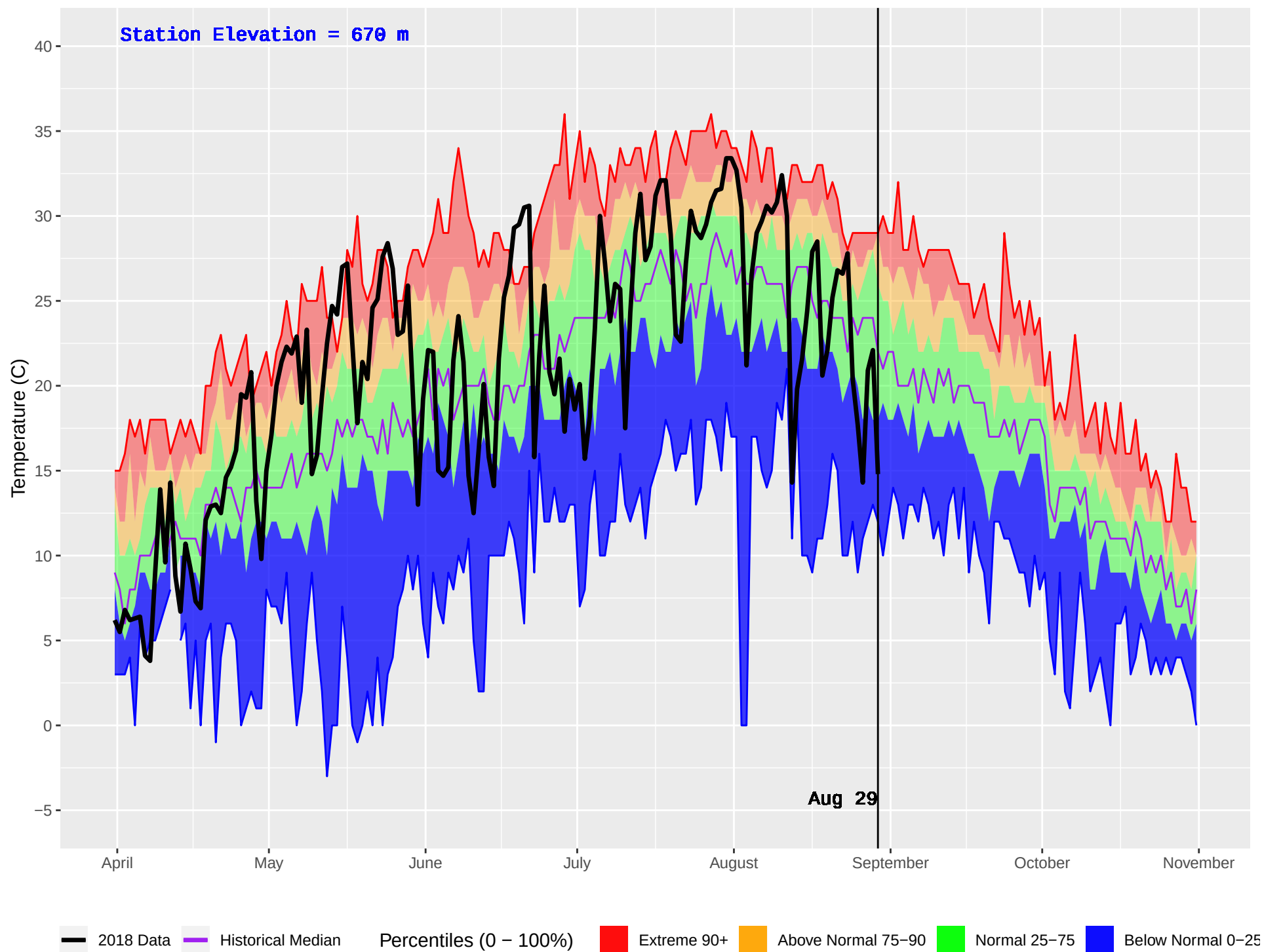
FINTRY (298) : Historical (1989–2016) and Current (2018) Daily Temperature
